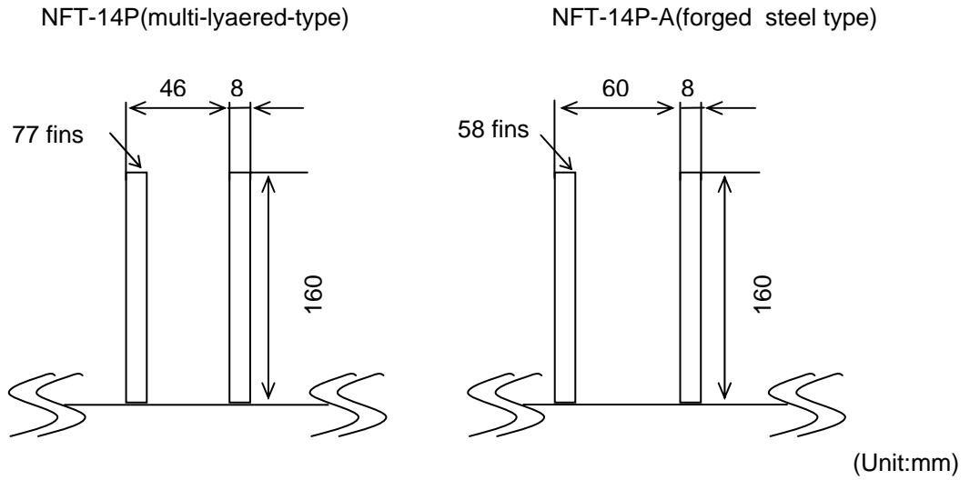
Fig.3 Change of Interval of Heat Removal fins
