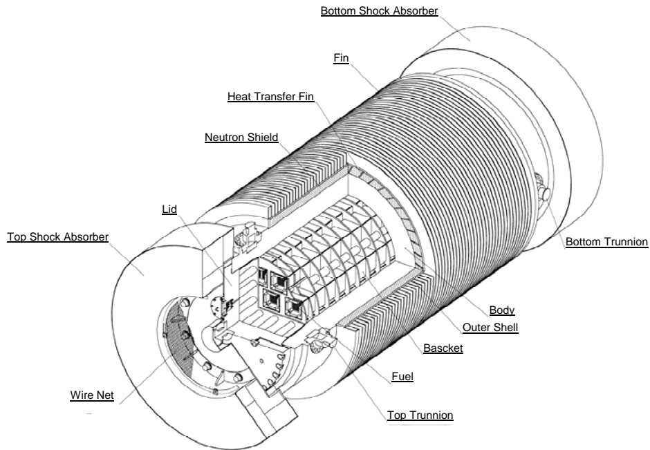
Fig.4 Overview of NFT-14P-A Cask
